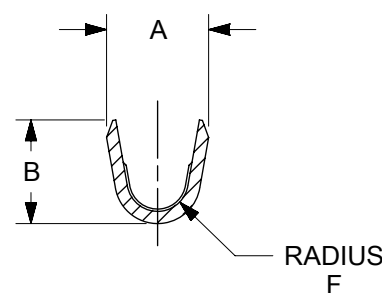
SECTION Y-Y WIRE BARREL
