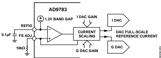
Figure 62. Reference Circuitry
