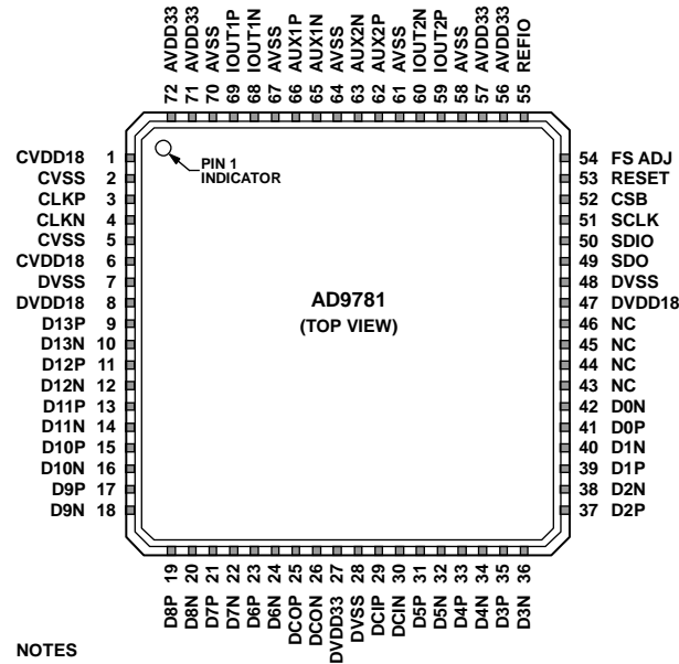
Figure 3. AD9781 Pin Configuration
