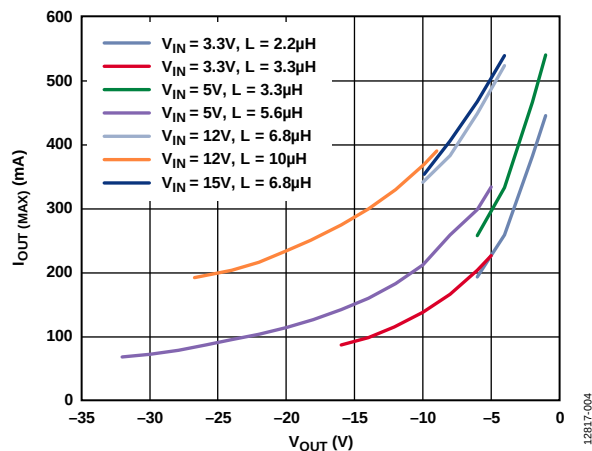
Figure 4. Maximum Output Current, f_{SW} = 2.4 \text{ MHz} , T_A = 25^\circ\text{C} , Based on Target of 70% I_{LIM}(\text{MIN})
