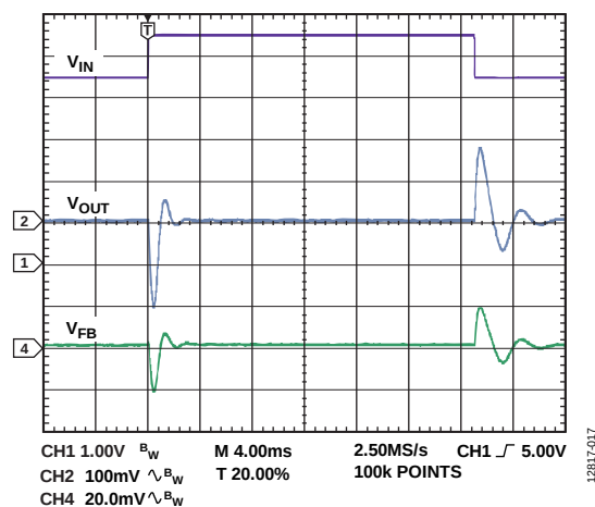
Figure 16. Line Transient Showing V_{IN} , V_{OUT} , and V_{FB} , V_{IN} = 4.5\text{ V} to 5.5\text{ V} Step, V_{OUT} = -5\text{ V} , R_{LOAD} = 300\Omega , f_{SW} = 1.2\text{ MHz} , T_A = 25^\circ\text{C}
