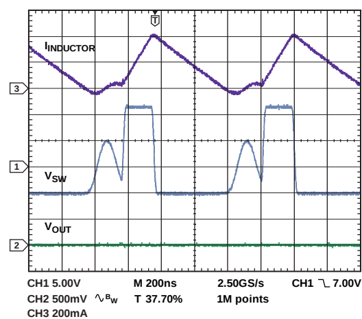
Figure 19. Discontinuous Conduction Mode Operation Showing Inductor Current ( I_{INDUCTOR} ), Switch Node Voltage ( V_{SW} ), and Output Ripple ( V_{OUT} ), V_{IN} = 12\text{ V} , V_{OUT} = -5\text{ V} , I_{LOAD} = 50\text{ mA} , f_{SW} = 1.2\text{ MHz} , T_A = 25^\circ\text{C}
