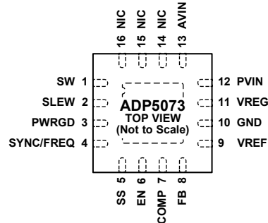
Figure 2. Pin Configuration
