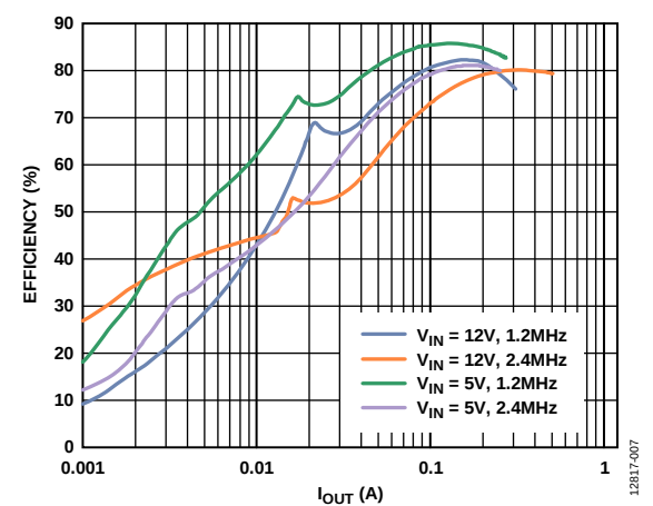
Figure 7. Efficiency vs. Current Load ( I_{OUT} ), V_{IN} = 12 \text{ V} and 5 \text{ V} , V_{OUT} = -15 \text{ V} , T_A = 25^\circ\text{C}
