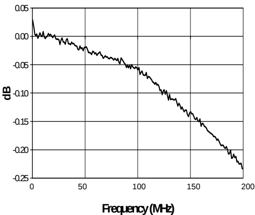
Amplitude Imbalance
