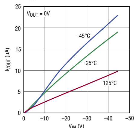
V_{OUT} Current vs Reverse V_{IN}
