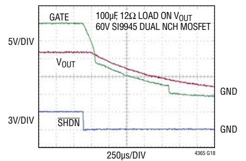
Turn-Off Timing
