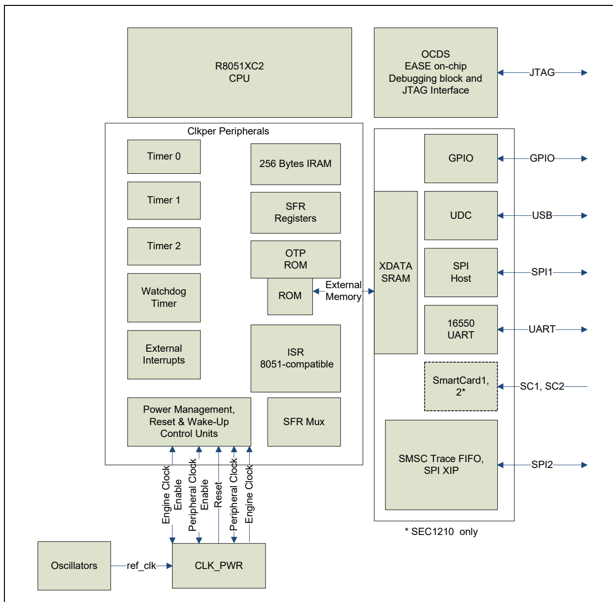
FIGURE 7-1: R8051XC2 Block Diagram
